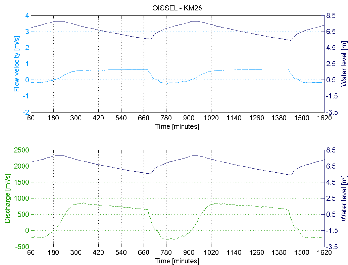
Figure A3 – Flow velocity (top) and discharge (bottom) from cubage at tidal station Oissel
